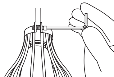
6. Evenly tighten cage bolts using supplied allen key
