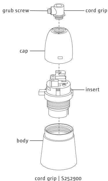
cord grip | S252900
